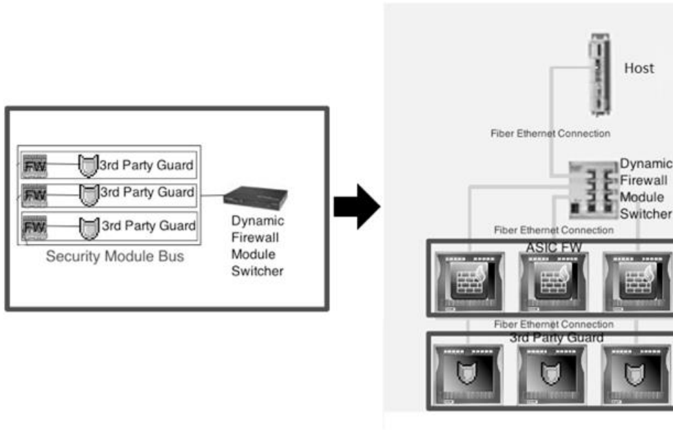
Figure 3: Bus structure of ASIC firewall security module
