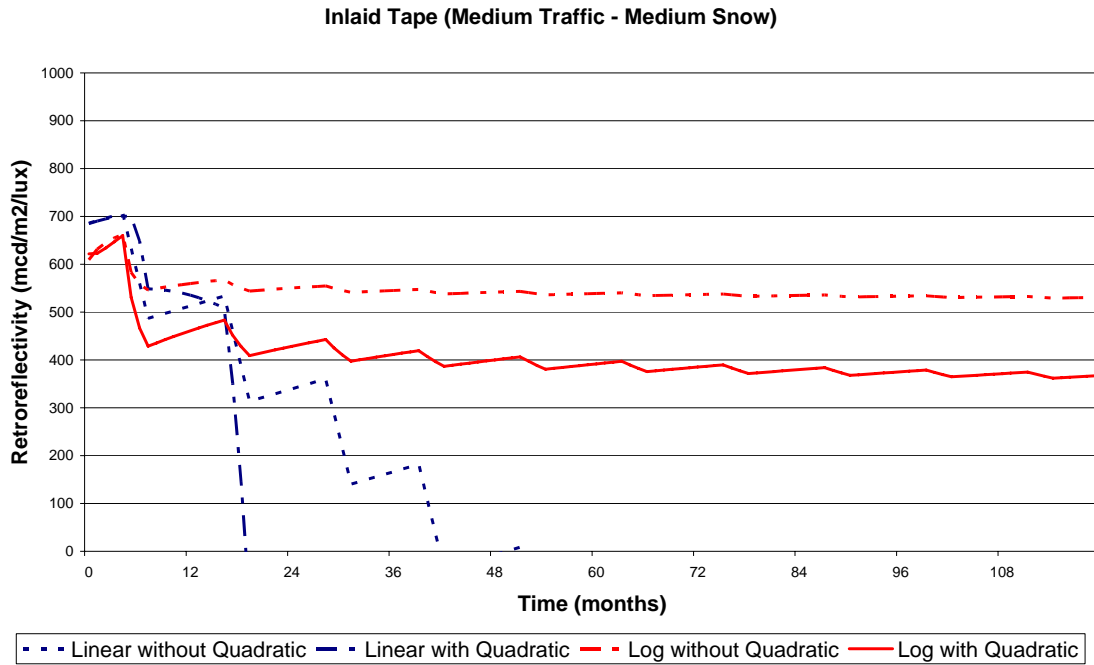
Figure 13. Regression Curves for Inlaid Tape (Medium Traffic & Medium Snow)
