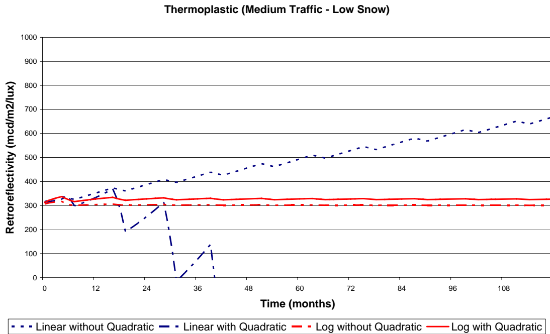
Figure 21. Regression Curves for Thermoplastic (Medium Traffic & Low Snow)
