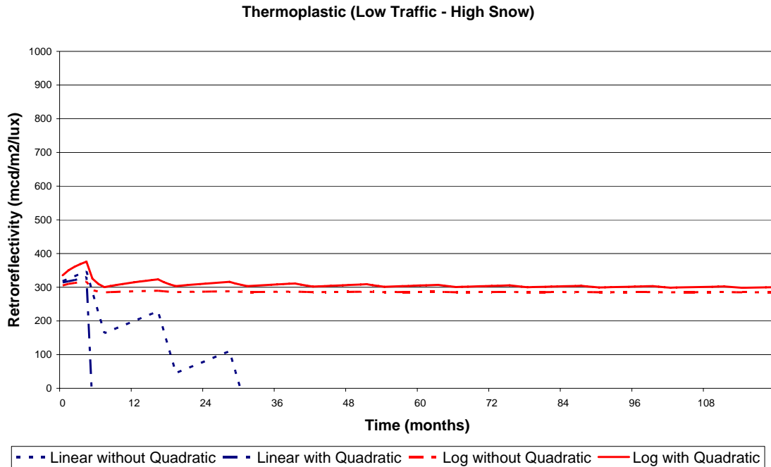
Figure 20. Regression Curves for Thermoplastic (Low Traffic & High Snow)
