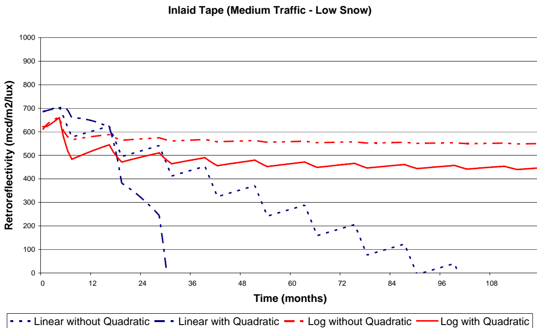
Figure 12. Regression Curves for Inlaid Tape (Medium Traffic & Low Snow)
