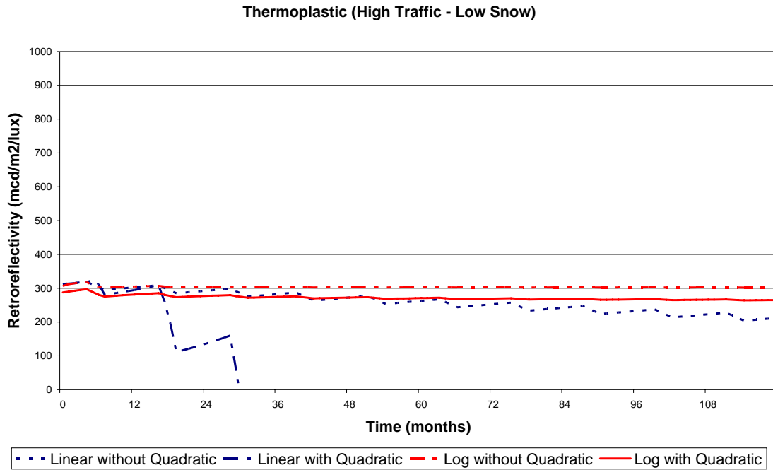
Figure 24. Regression Curves for Thermoplastic (High Traffic & Low Snow)
