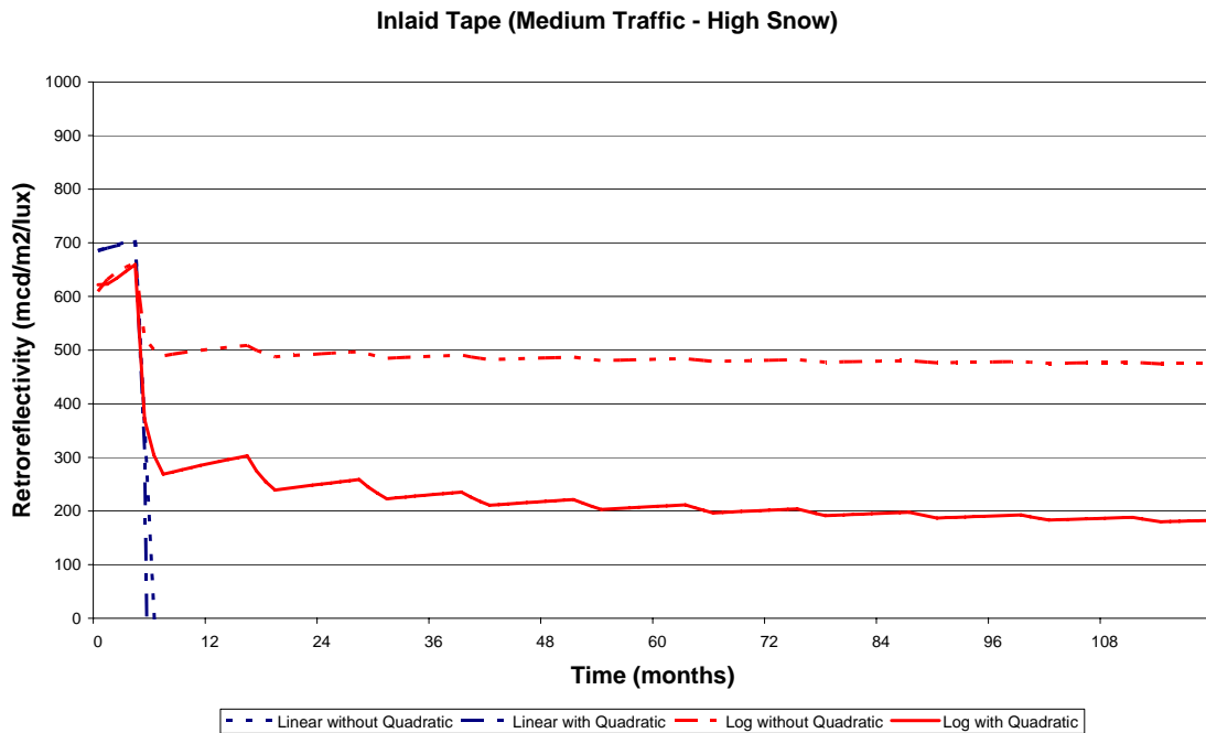
Figure 14. Regression Curves for Inlaid Tape (Medium Traffic & High Snow)
