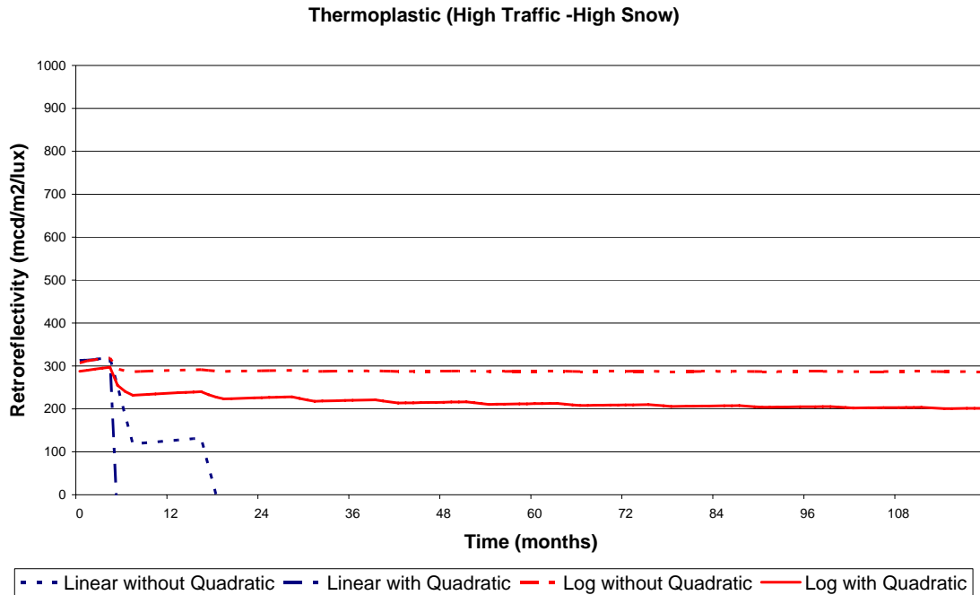
Figure 26. Regression Curves for Thermoplastic (High Traffic & High Snow)
