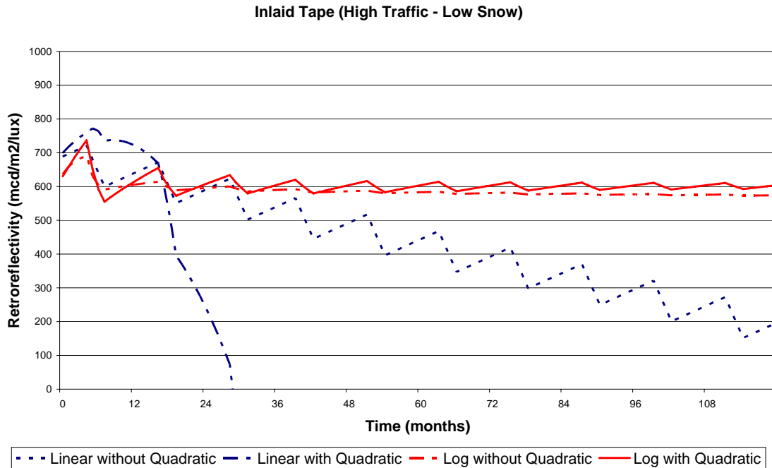
Figure 15. Regression Curves for Inlaid Tape (High Traffic & Low Snow)
