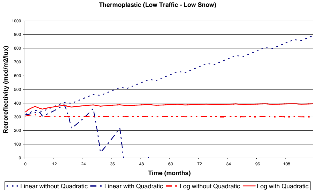
Figure 18. Regression Curves for Thermoplastic (Low Traffic & Low Snow)
