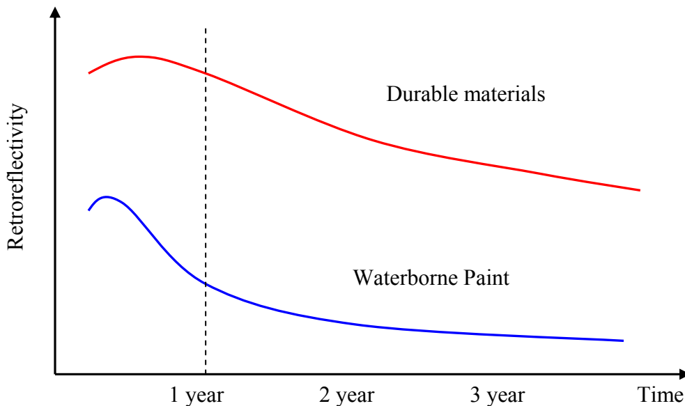
Figure 6. Typical Retroreflectivity Curves for the Different Pavement Marking Materials
