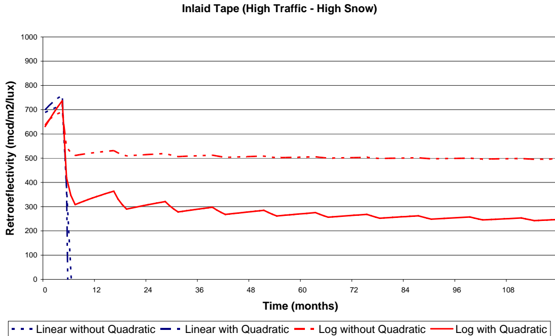
Figure 17. Regression Curves for Inlaid Tape (High Traffic & High Snow)
