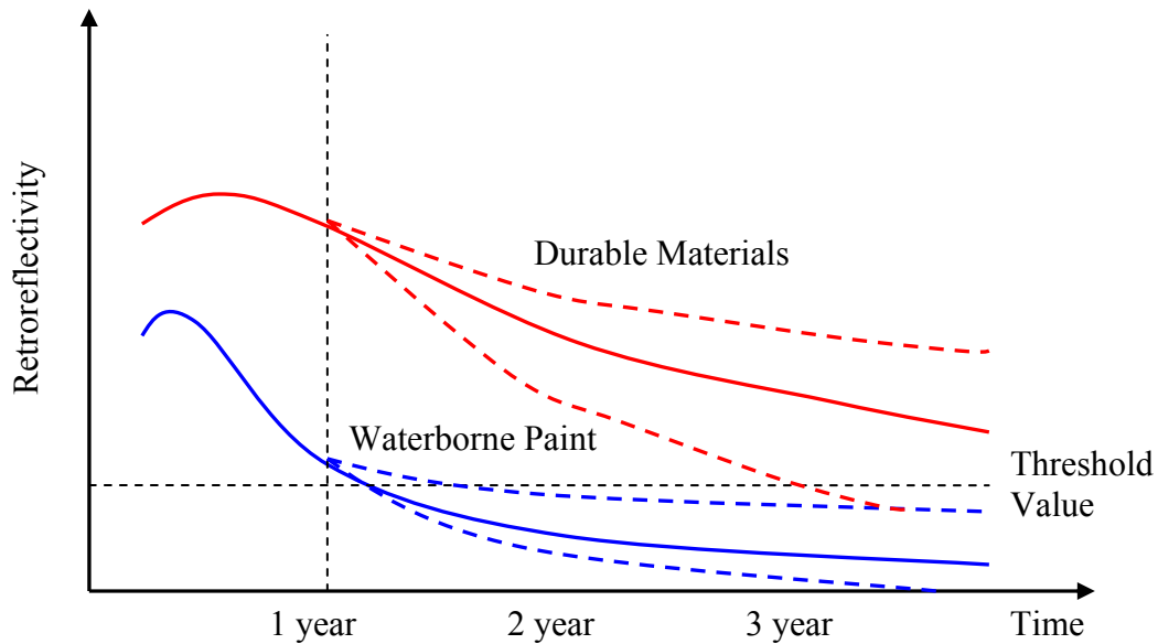
Figure 8. Different Life Cycles with Different Estimation Curves
