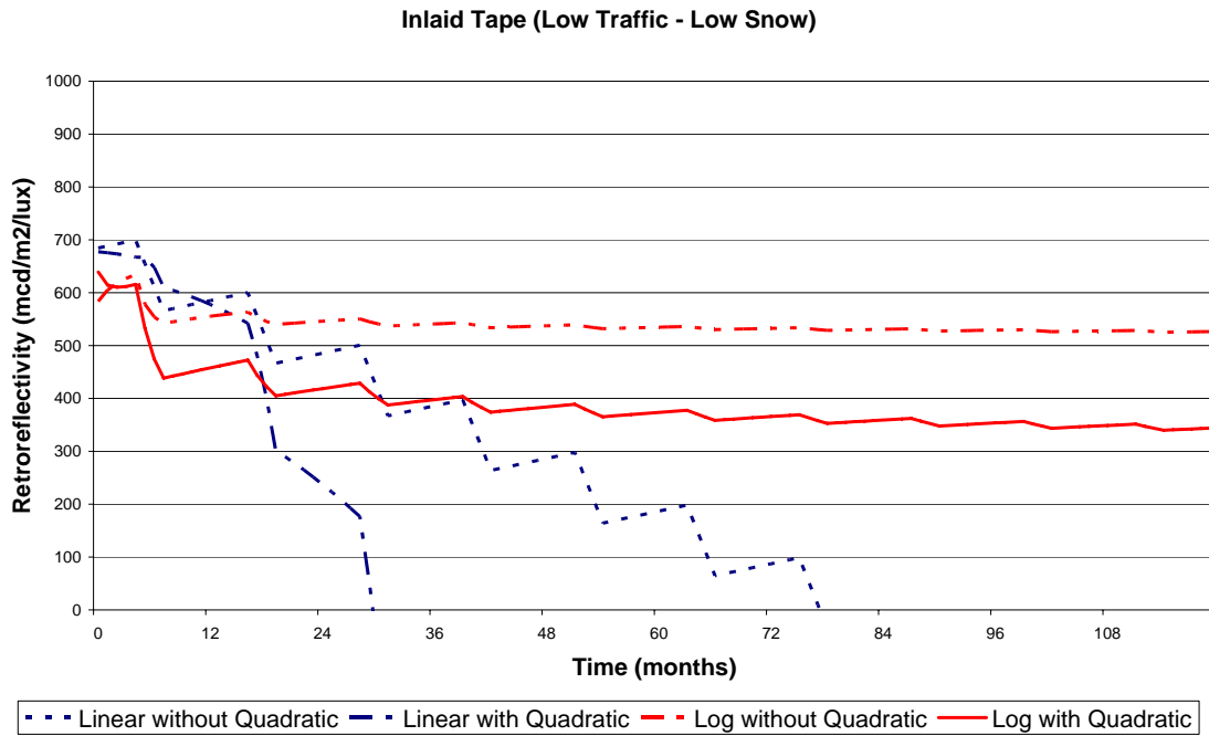
Figure 9. Regression Curves for Inlaid Tape (Low Traffic & Low Snow)
