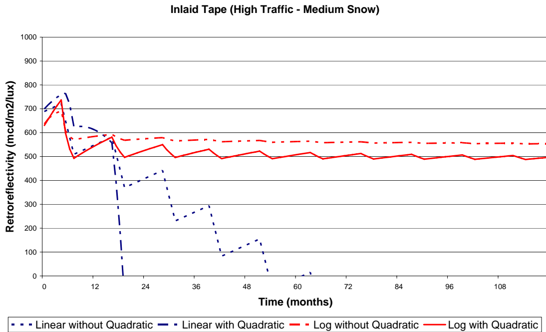
Figure 16. Regression Curves for Inlaid Tape (High Traffic & Medium Snow)
