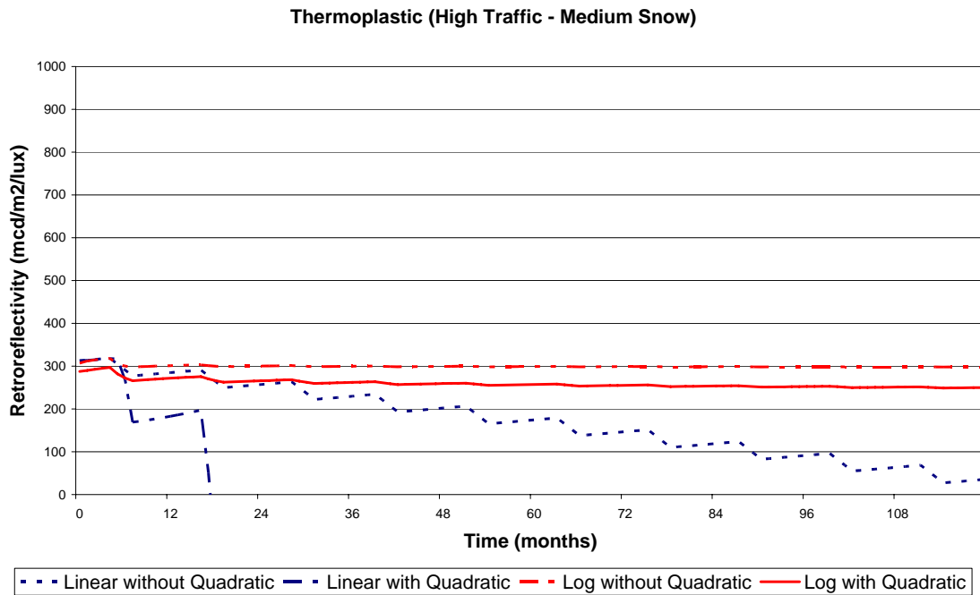
Figure 25. Regression Curves for Thermoplastic (High Traffic & Medium Snow)
