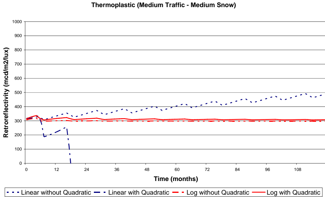
Figure 22. Regression Curves for Thermoplastic (Medium Traffic & Medium Snow)
