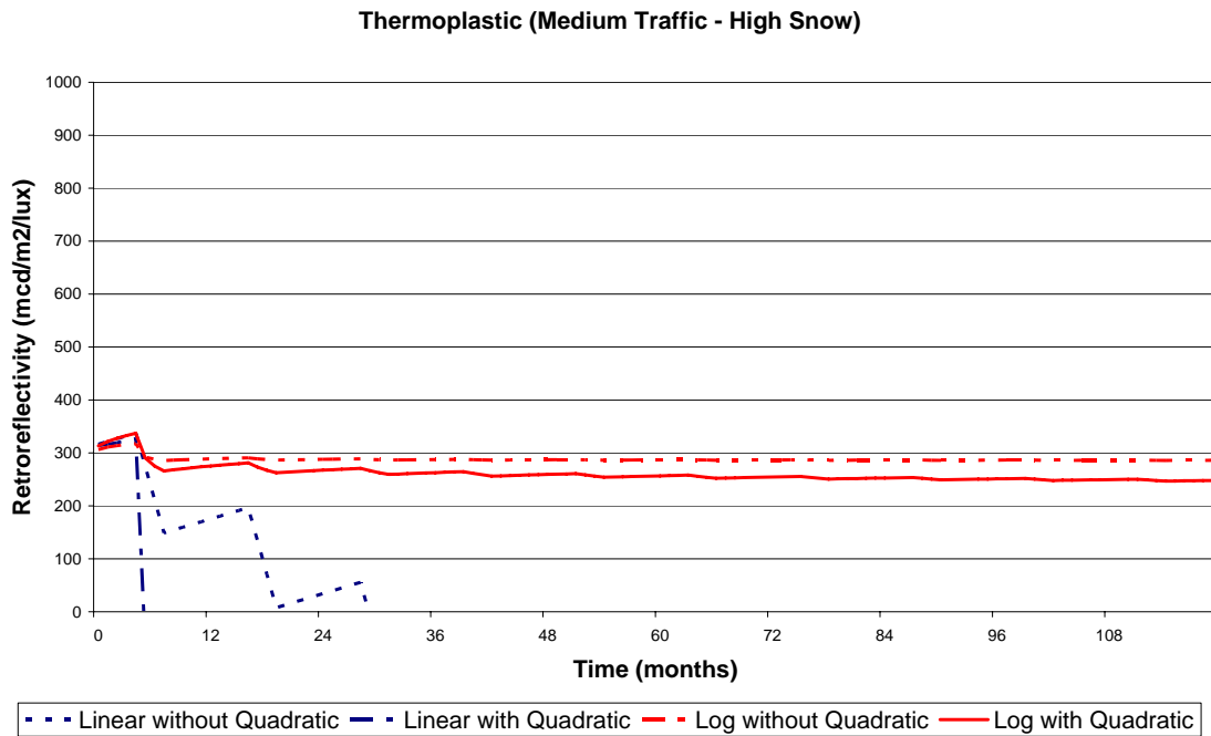
Figure 23. Regression Curves for Thermoplastic (Medium Traffic & High Snow)
