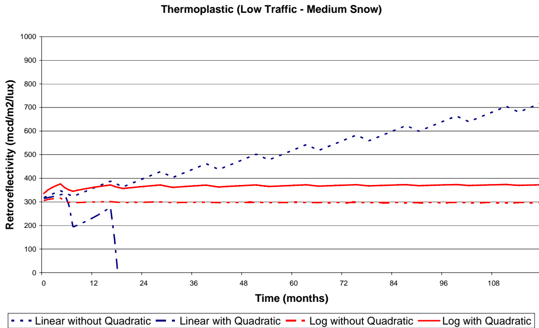
Figure 19. Regression Curves for Thermoplastic (Low Traffic & Medium Snow)
