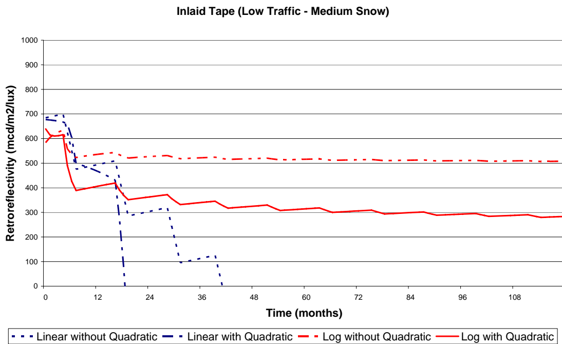
Figure 10. Regression Curves for Inlaid Tape (Low Traffic & Medium Snow)
