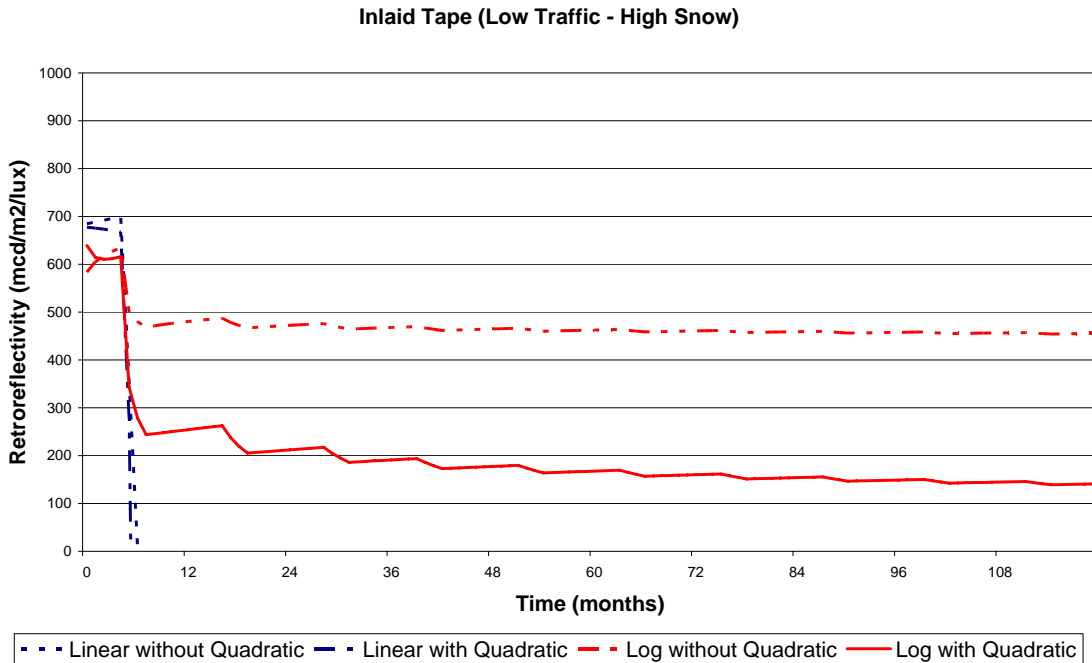
Figure 11. Regression Curves for Inlaid Tape (Low Traffic & High Snow)
